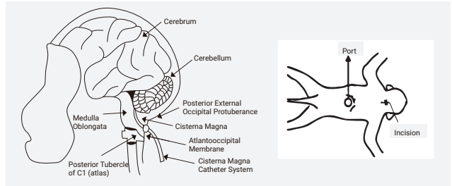
Position of the cistern magna cannulation catheter and port
